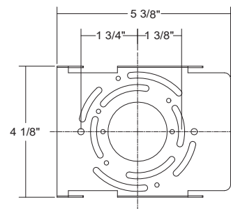
Mounting back plate
