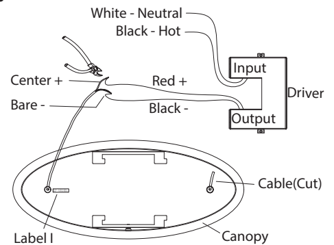
Fig.3 Driver Wires
